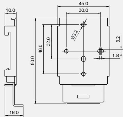
H type Rail bracket ( HS-BR-1 )
