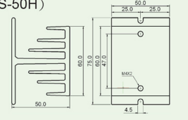
Heat sink (HS-50H)
