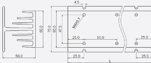
H type
