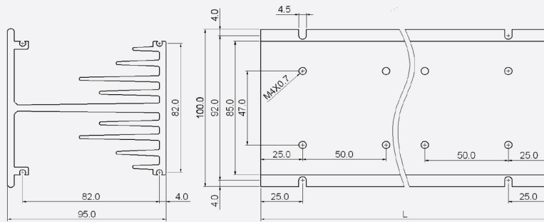
Standard type
